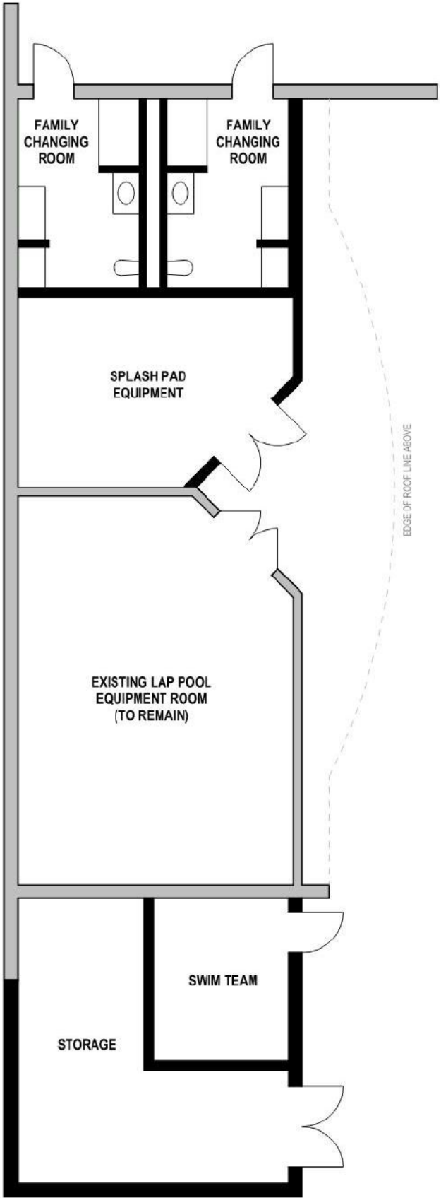
CONCEPT FLOOR PLAN
